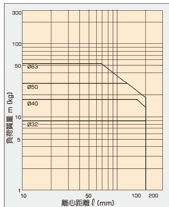
● (H) 50行程以上, V = 200\text{mm/s}
