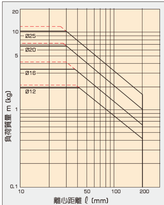
● (E) 30行程未滿, V = 200\text{mm/s}
